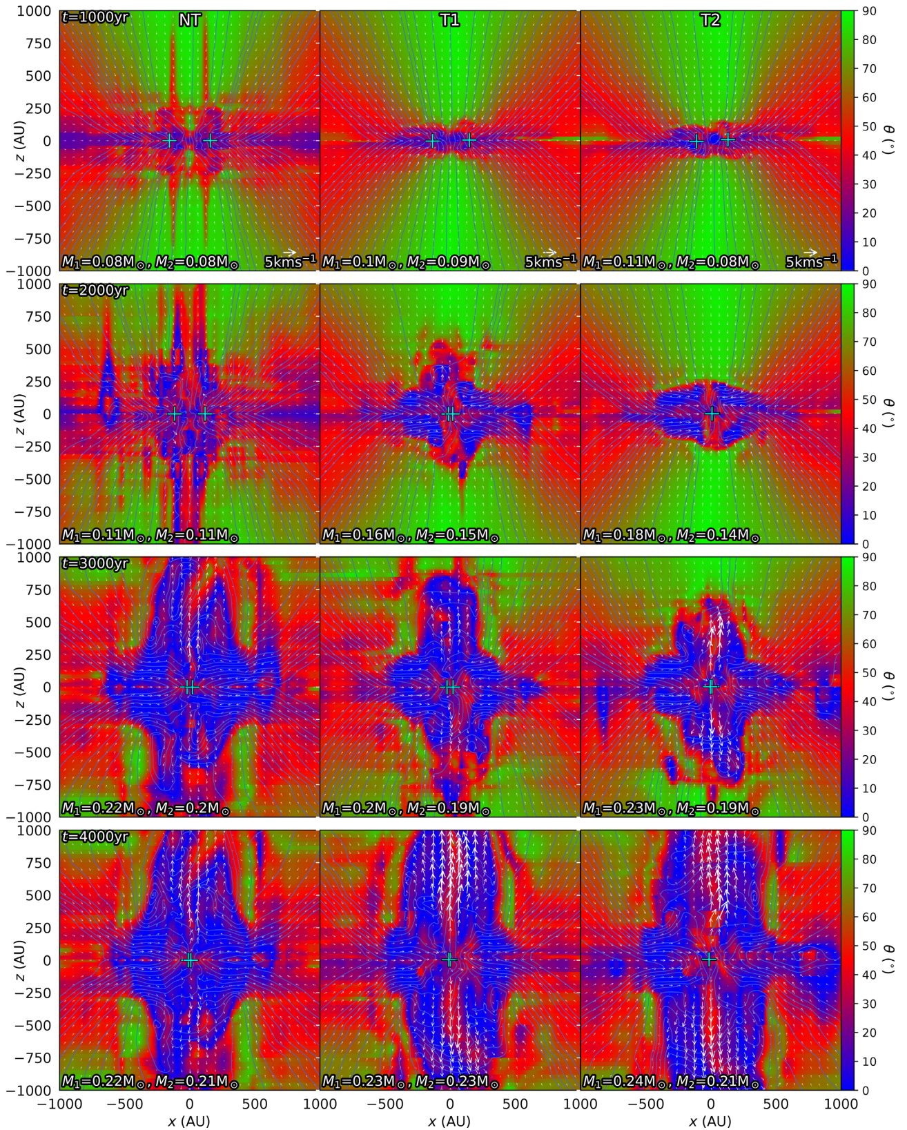
Figure 4. Same as Fig. 1, but shows volume-weighted slices of the magnetic field angle to the xy -plane.
