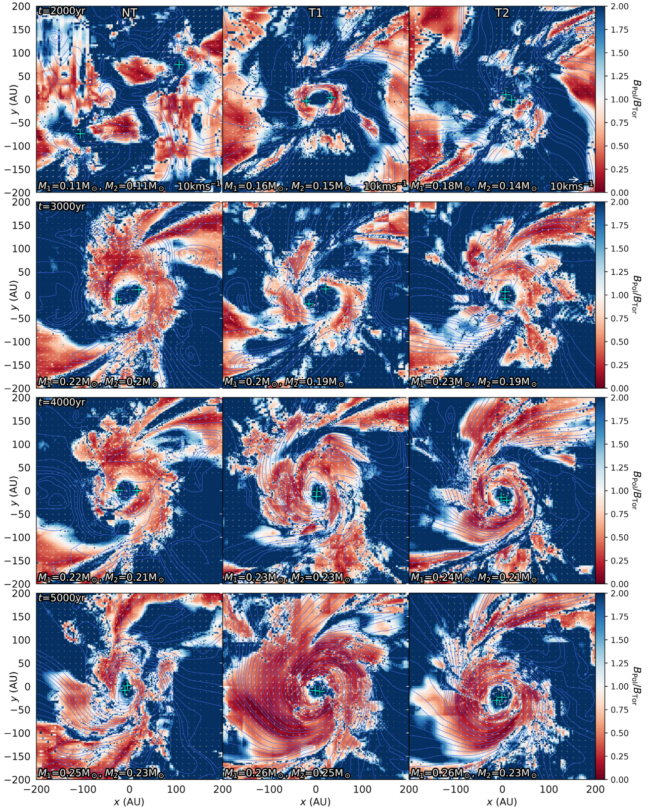
Figure 7. Same as Fig. 2, but shows volume-weighted slices of the ratio of the poloidal component ( B_{\text{pol}} ) to the toroidal component ( B_{\text{tor}} ) of the magnetic field.
