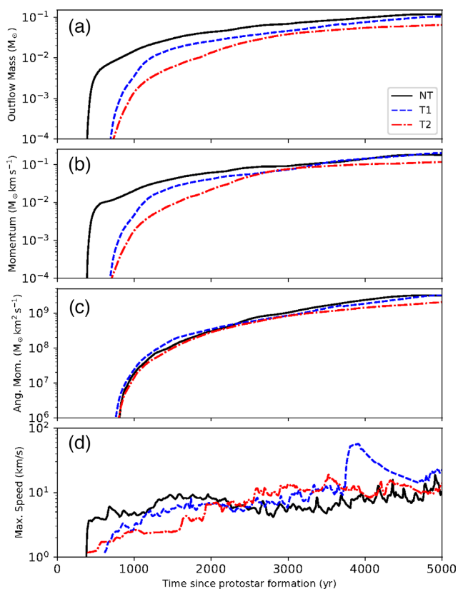
Figure 6. Time evolution of the outflow quantities measured from cylinders of radius 500 au and height 500 au placed at 100 au above and below the disc z = 0 plane. Panel (a): outflowing mass, defined as mass within cells with v_z away from the disc. Panel (b): linear momentum of the outflowing gas. Panel (c): angular momentum of the outflowing gas calculated around the centre of mass of the system. Panel (d): the speed of the cell with the maximum speed within the measuring volume.
