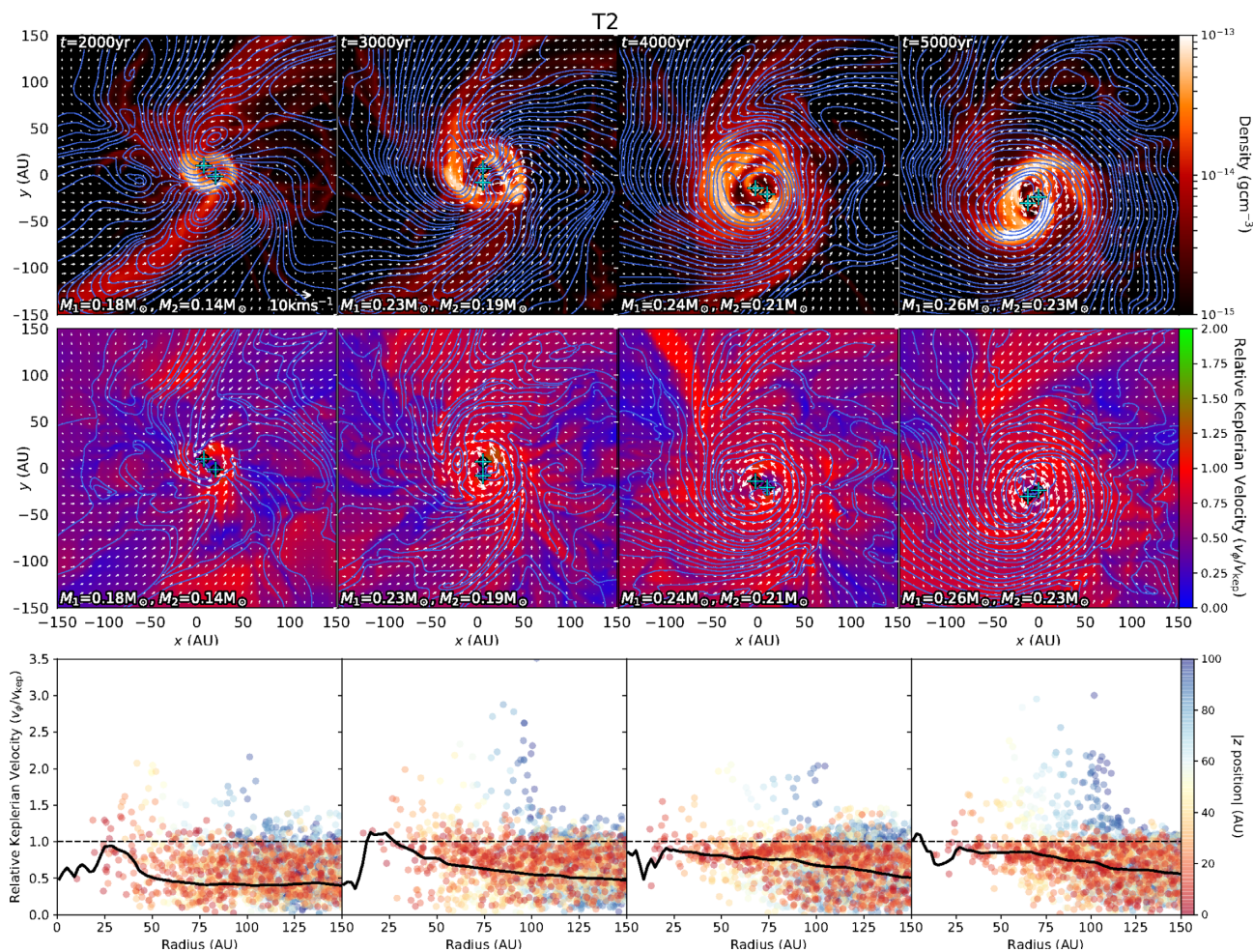
Figure 10. Same as Fig. 8, but for T2.
