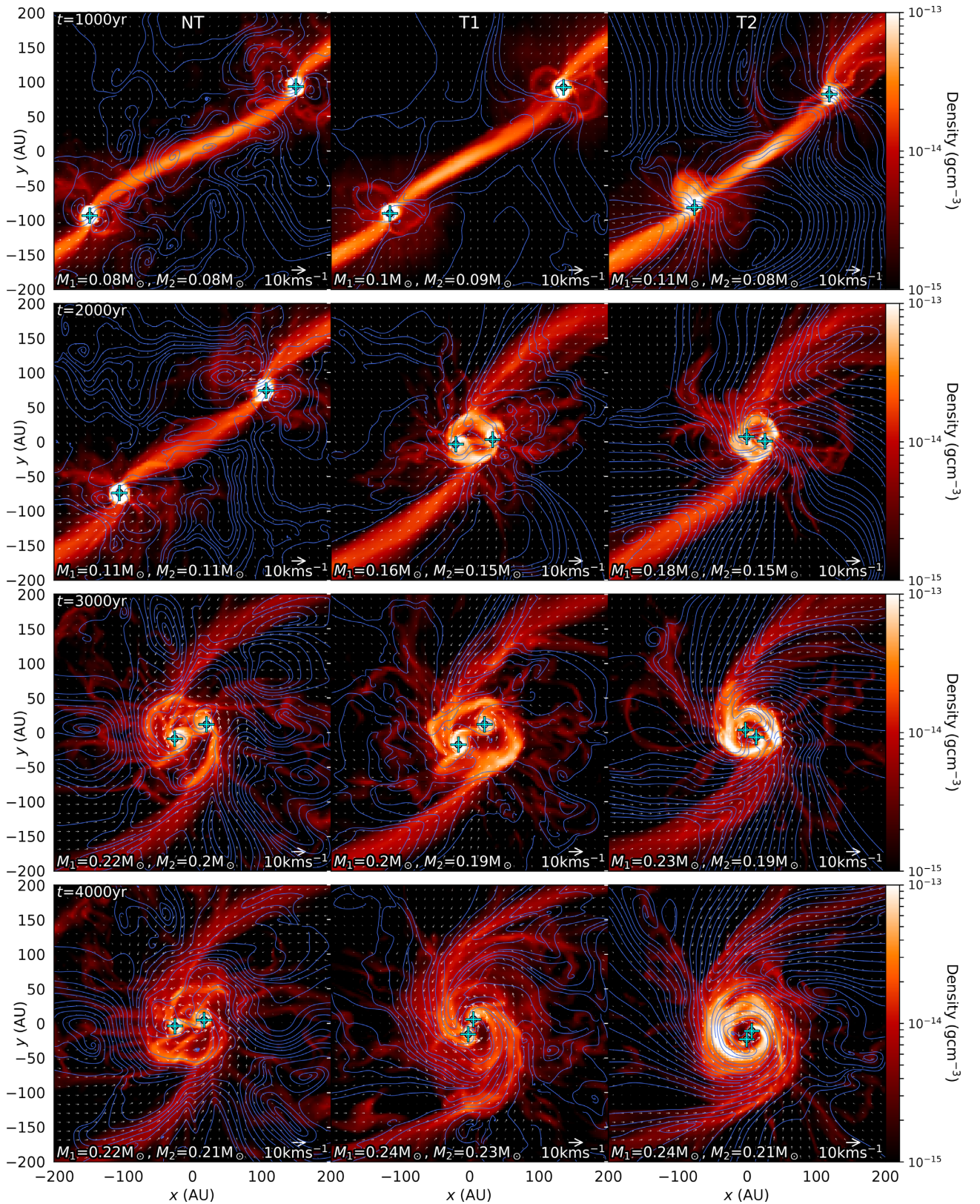
Figure 2. Same as Fig. 1, but for 100 au thick slices along the z = 0 plane of the simulation box.
