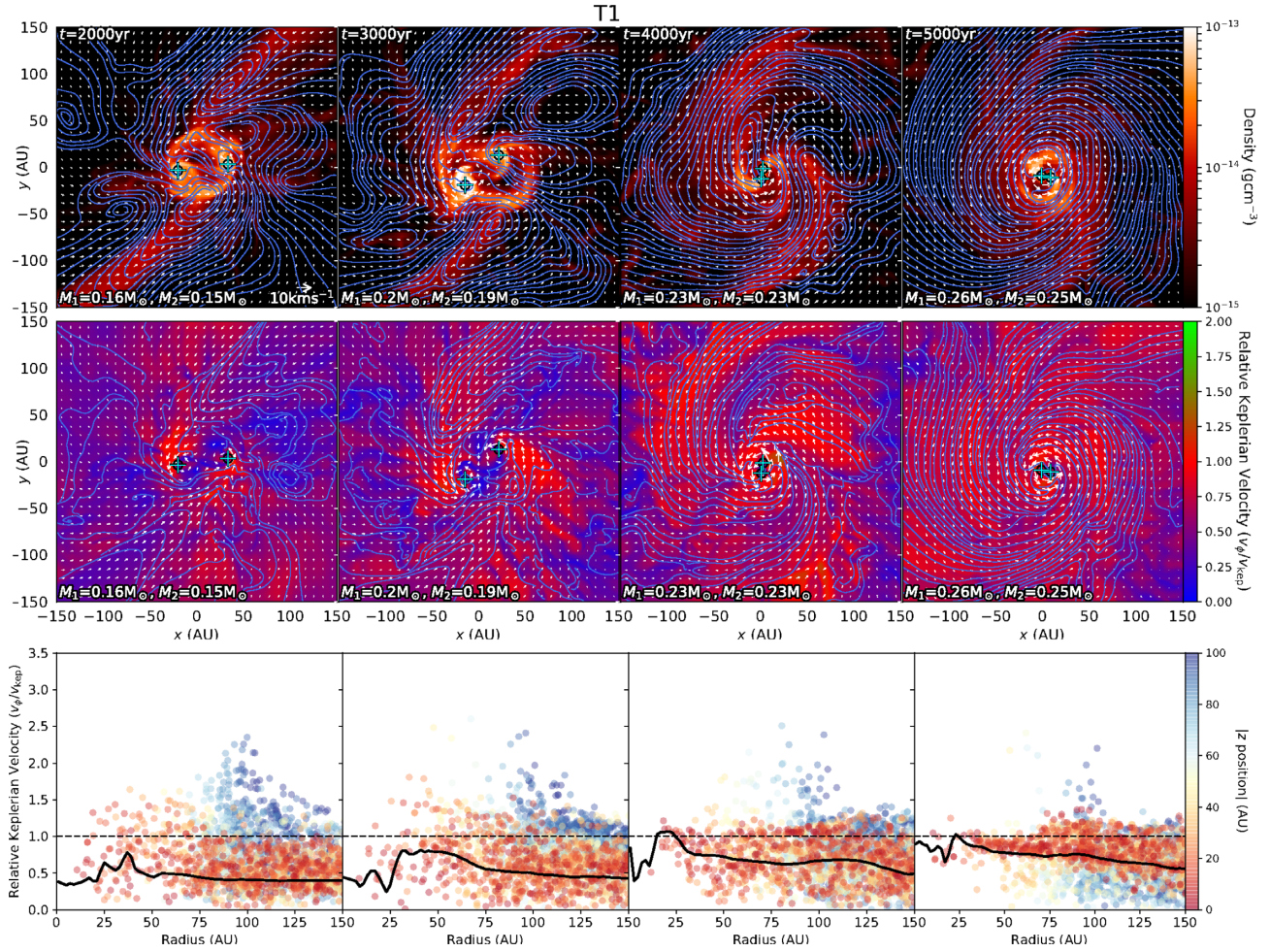
Figure 9. Same as Fig. 8, but for T1.
