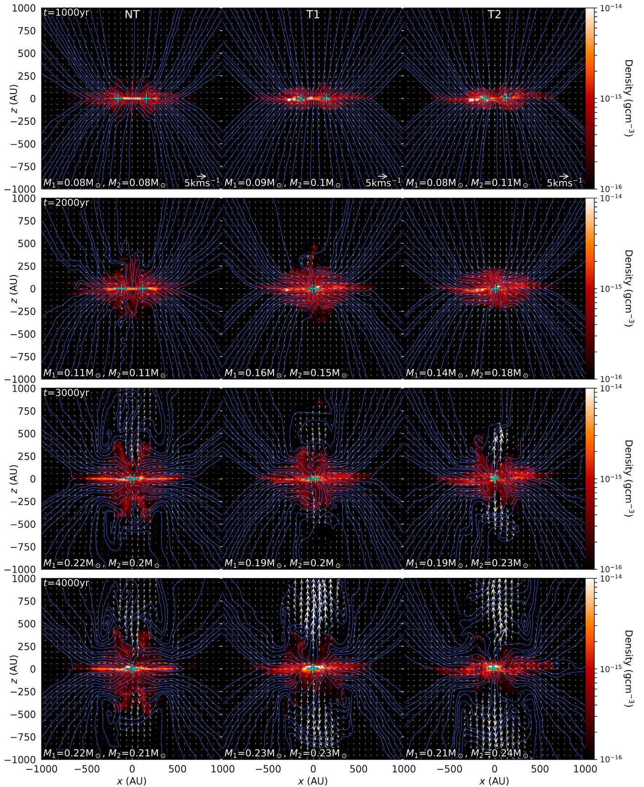
Figure 1. 300 au thick volume-weighted slices orientated along the dense accretion streams such that the slice captures the dense material and two sink particles for NT (left), T1 (middle), and T2 (right). Each row progresses at 1000 yr intervals since the first protostar formation. The thin lines show the magnetic field, and the arrows indicate the velocity field. Crosses show the position of the sink particles. The mass accreted by the sink particles in the simulations is indicated on the bottom left of each panel.
