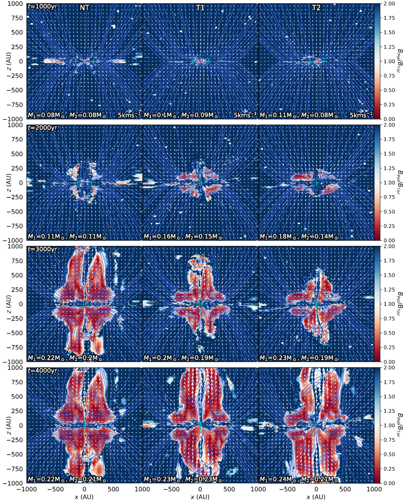
Figure 5. Same as Fig. 1, but shows volume-weighted slices of the ratio of the poloidal component ( B_{\text{pol}} ) to the toroidal component ( B_{\text{tor}} ) of the magnetic field.
