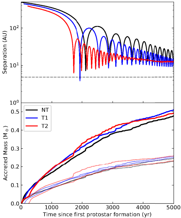
Figure 3. Shows the evolution of the binary separation (top) and accreted mass (bottom) since protostar formation of the first sink particle for the NT, T1, and T2 cases in black, blue, and red, respectively. In the plot of the accreted mass, the transparent thin lines trace the mass of the individual components and the thick opaque lines traces the total accreted mass.
